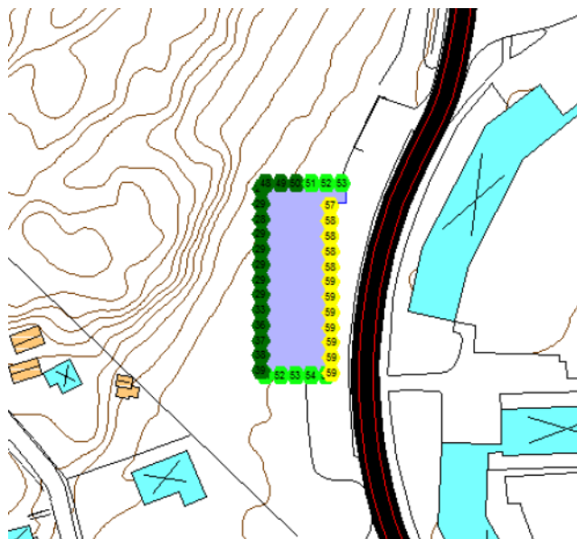
Figur 16, Fasadljudnivåer.
