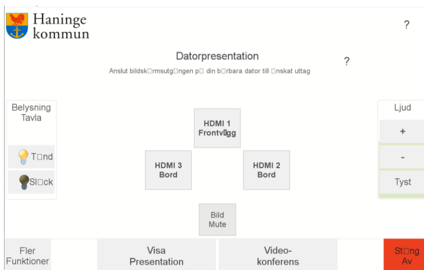
Figur 3 Visa Presentation
